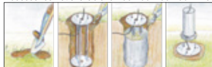
Root Mounting Kit code 00A400
